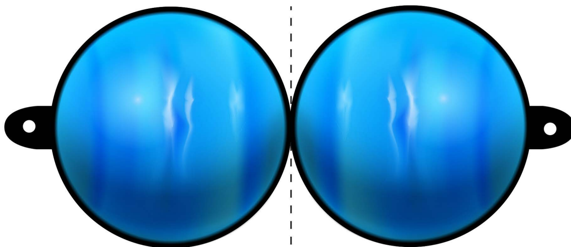
Neptune
